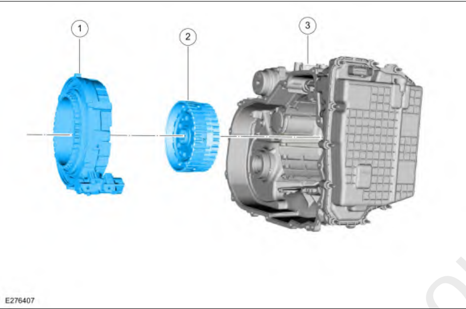
Hydraulic Selectable One-Way Clutch (SOWC) Assembly
